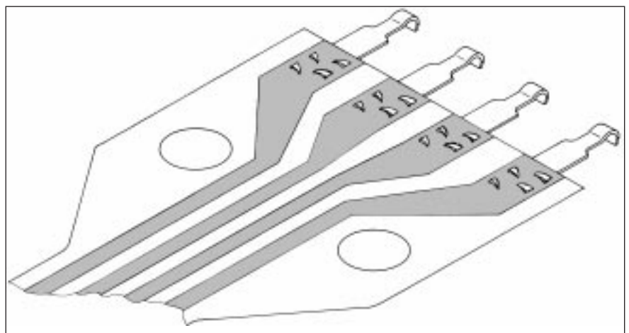
A 4 x FFC solder contact connected to the sensor foil after bending the tips of the tabs.
