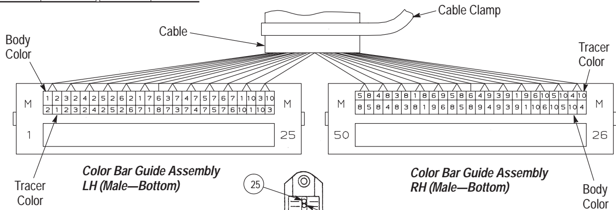
Wire and Connector Placement for Terminating Receptacle Connector
