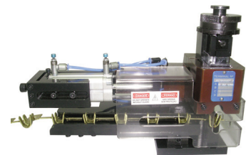
Large Wire Applicator
